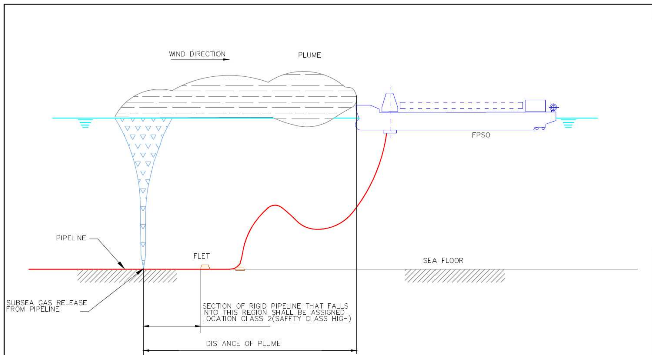
Figure 2. Consequence of subsea gas release.
