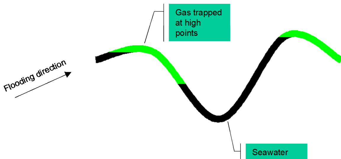
Figure 5. Entrapment of gas at high points in pipeline.
