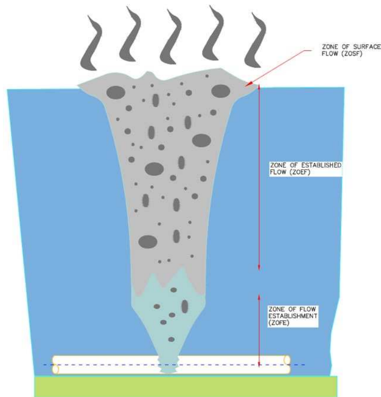
Figure 3. Gas Release from a Rupture Subsea Pipeline [43–46].
