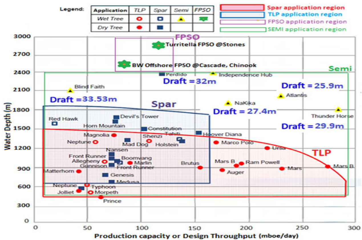
Figure A6. Map of breakdown of Application envelopes for deep-water platforms in the Gulf of Mexico {Illustrated by: Author 1—C.V.A.}.
