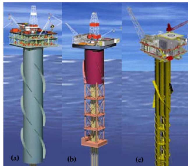
Figure 13. Types of Spar Platform: (a) Classic (b) Truss (c) Cell.
