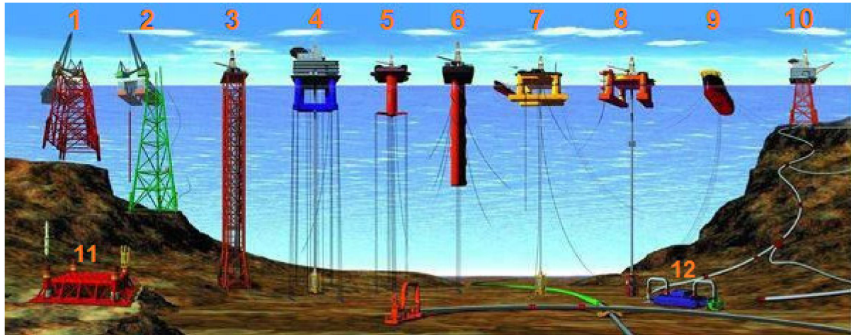
Figure 1. Different types of deep-water offshore production facilities, showing (1,2) conventional fixed platforms {150–412 m}; (3) compliant tower {457–914 m}; (4,5) tension leg platform (TLP) {457–2134 m}; (5) mini tension leg platform (TLP); (6) Truss SPAR {610–3048 m}; (7,8) semisubmersibles {457–1920 m}; (9) floating production, storage and offloading (FPSO) unit {1345–1500 m}; and (10) jacket platform {150–412 m}; and (11) subsea completion and tieback to a host facility, and (12) subsea manifold. (Adapted from public domain source, with permission obtained to re-use image; Courtesy: National Oceanic and Atmospheric Administration, NOAA).
