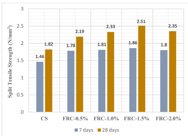
Fig. 5. Split tensile strength at 7 and 28 days with varying percentages of kenaf and polypropylene fibre.
