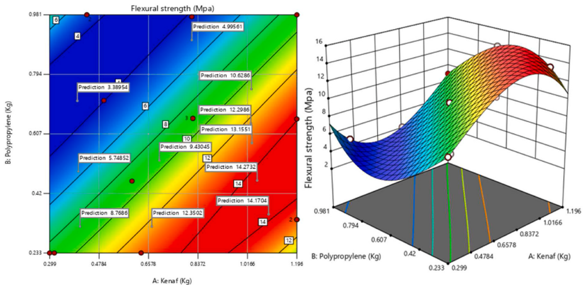
Fig. 9. Response surface plot for the influence of kenaf and polypropylene on the flexural strength of hybrid concrete.
