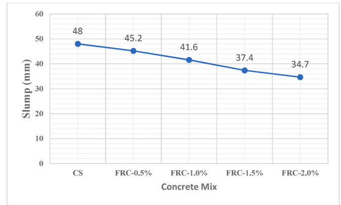
Fig. 3. Variation of slump with fibre content.
