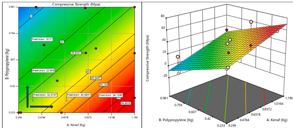
Fig. 7. Response surface plots for the influence of kenaf and polypropylene fibres on compressive strength.
