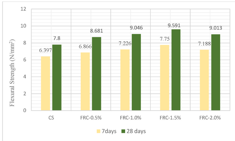
Fig. 6. Flexural Strength at 7 and 28 days with varying percentages of kenaf and polypropylene fibre.
