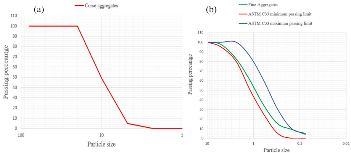
Fig. 2. Grain size distribution (a) Coarse aggregate (b) Fine aggregate.
