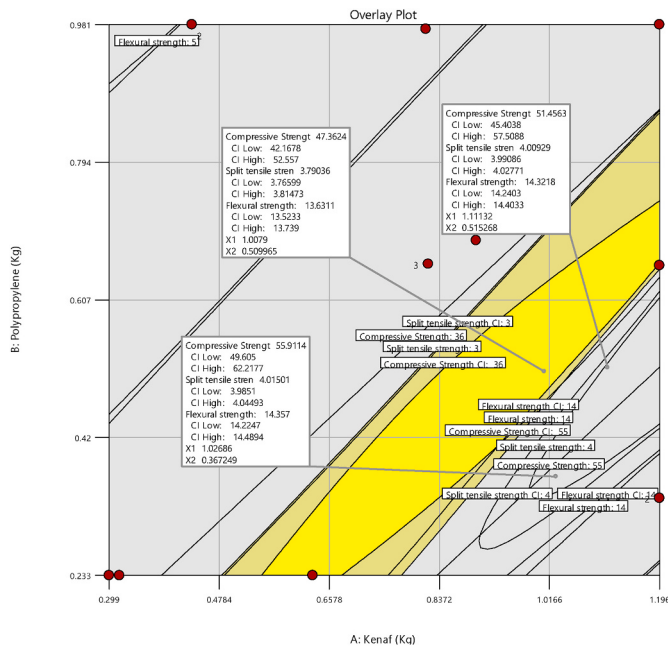
Fig. 11. Graphical Optimised plots of combined responses.
