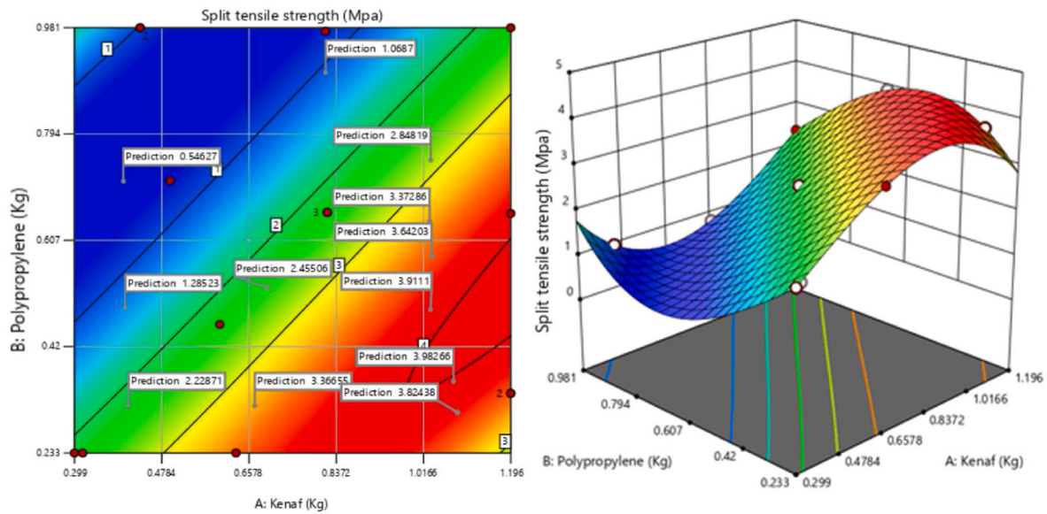
Fig. 8. Response surface plot for the influence of kenaf and polypropylene on split tensile strength of hybrid concrete.
