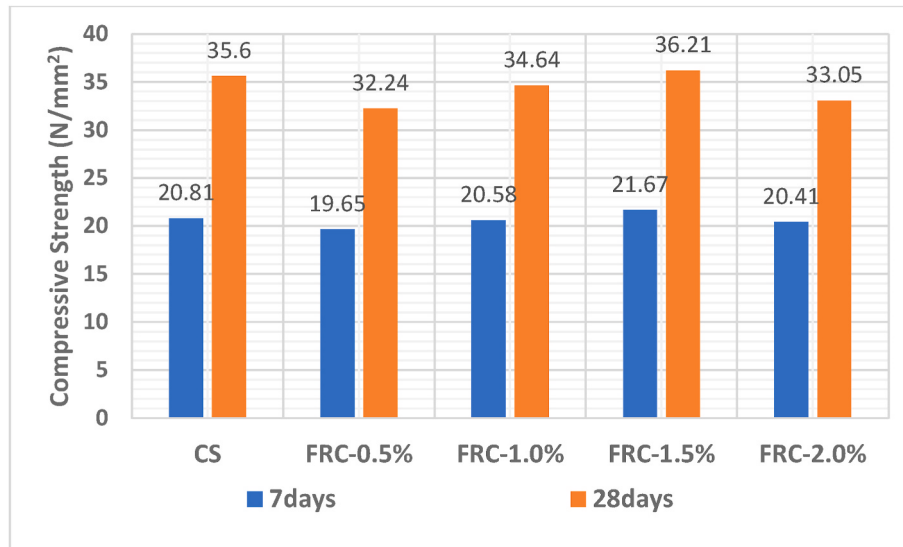
Fig. 4. Compressive strength at 7 days with varying percentages of kenaf and polypropylene fibre.
