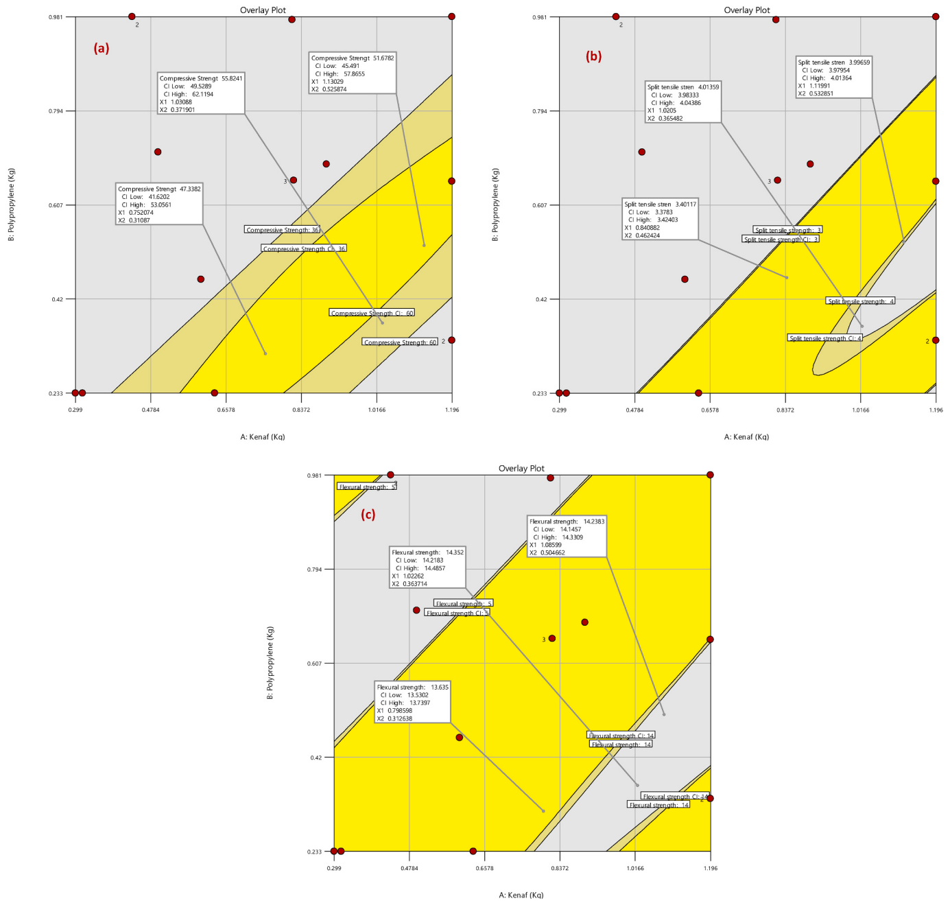
Fig. 10. Overlay plots of predicted responses (a) compressive strength (b) Split tensile strength (c) Flexural strength.
