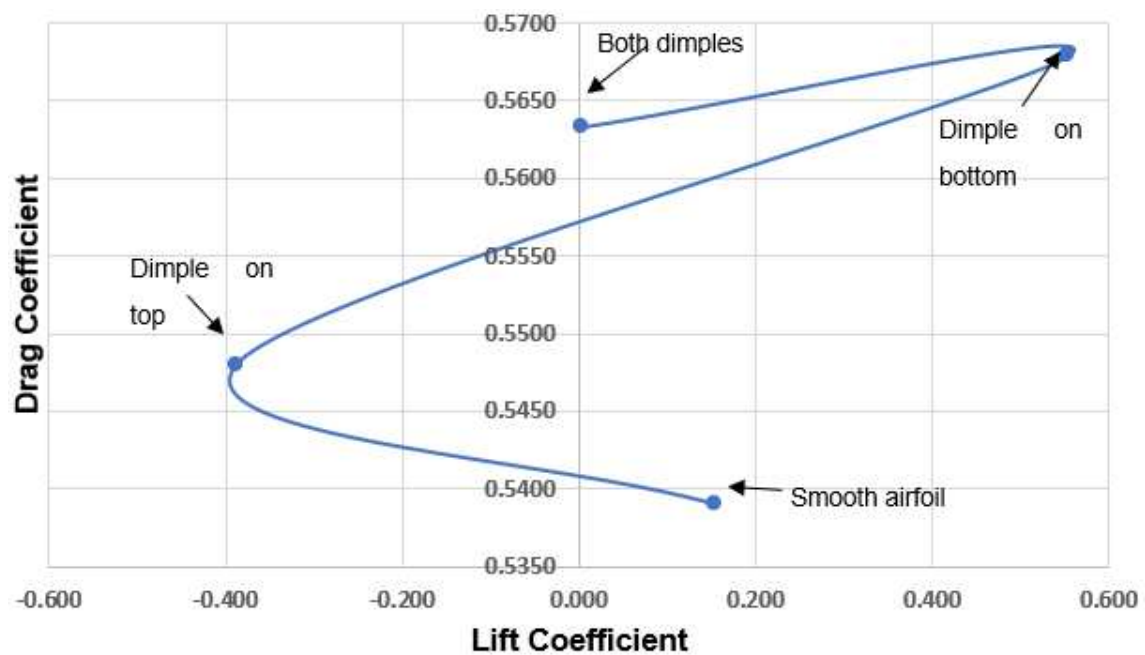
Figure 15. The relationship between lift and drag coefficients on an aerofoil with an ellipse-shaped dimple.
