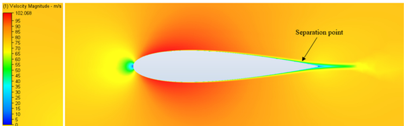
Figure 13. NACA 0017 aerofoil acting at 0^\circ AOA showing Separation point over.
