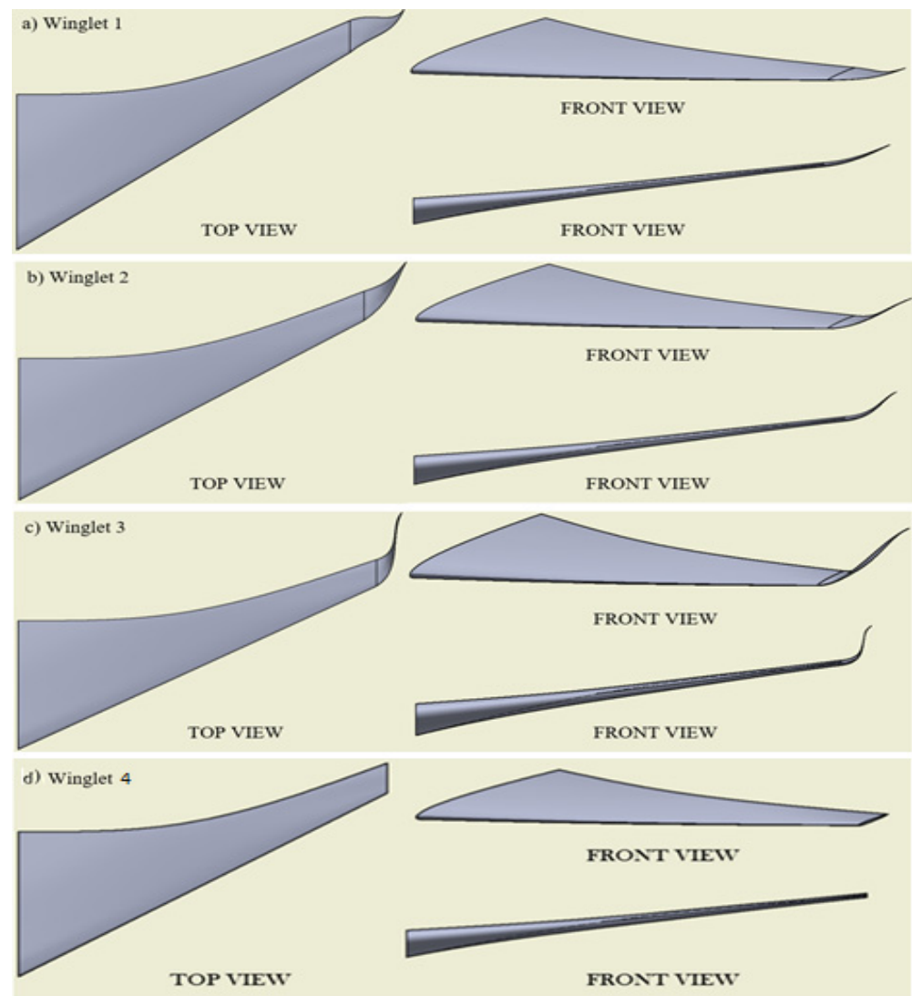
Figure 2. Winglet designs (a) 20^\circ cant angle, extending 4 m from main wing, height of 1 m (b) 45^\circ cant angle, extending 3 m, with a height of 2 m (c) 65^\circ cant angle, extending 2 m, with a height of 3 m (d) 0^\circ for the Boeing 787-9 Dreamliner wing.
